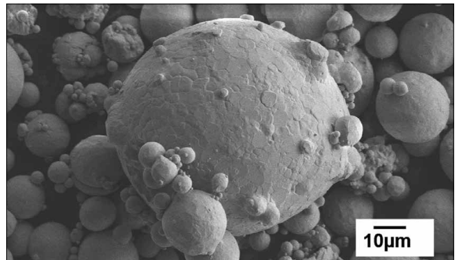
Pulver-Material: CuCrZr
