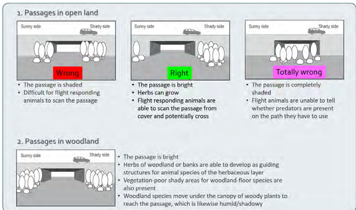
Fig. 21: Trees and bushes at narrow underpasses, favourable and unfavourable arrangements differ in woodland and in open land
