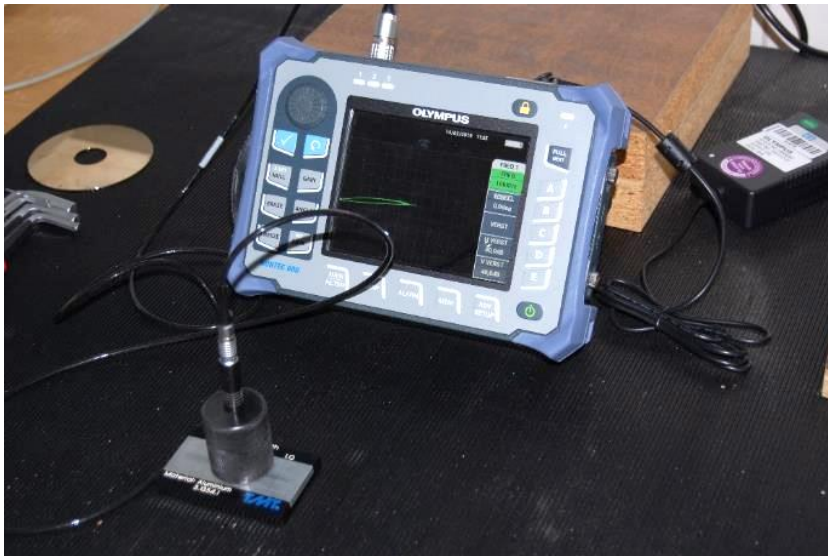
Olympus Nortec 600
